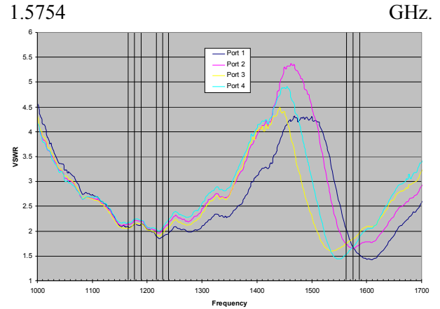
Figure 2: Measured VSWR of Triple Frequency GPS Trap Loaded Inverted L Antenna Array
