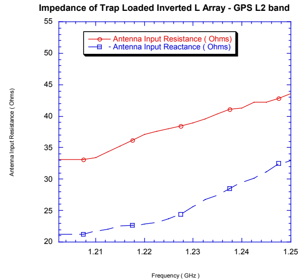
Figure 3b: Measured Input Impedance in the L_2 Band
