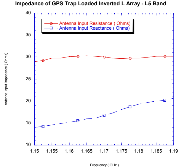
Figure 3a: Measured Input Impedance in the L_5 Band
