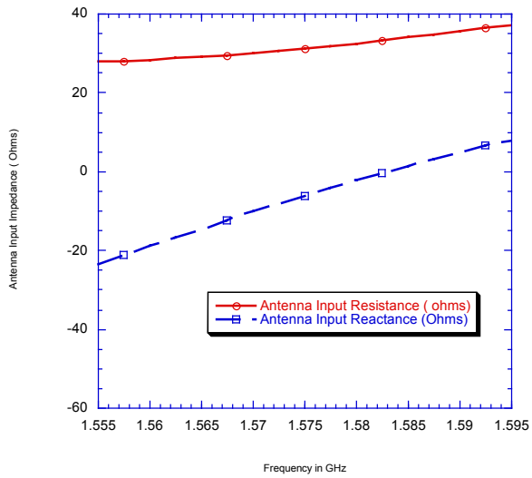
Impedance of GPS Trap Loaded Inverted L Array - GPS L1 Band
