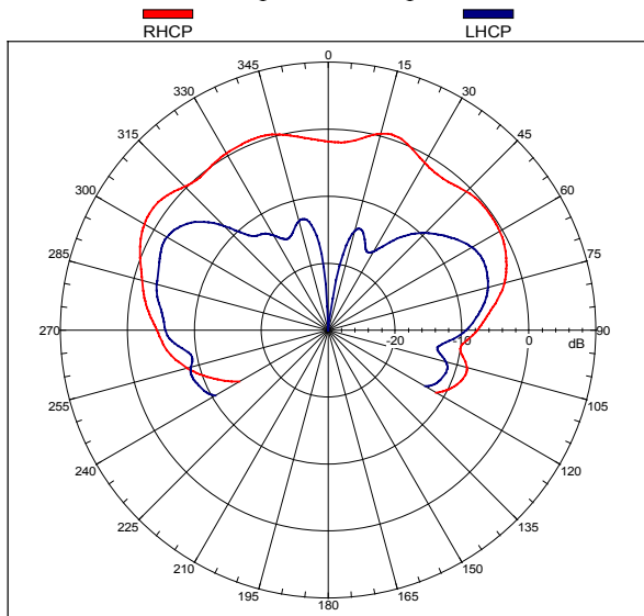
Far-field amplitude of Dsph231a2.nsi
