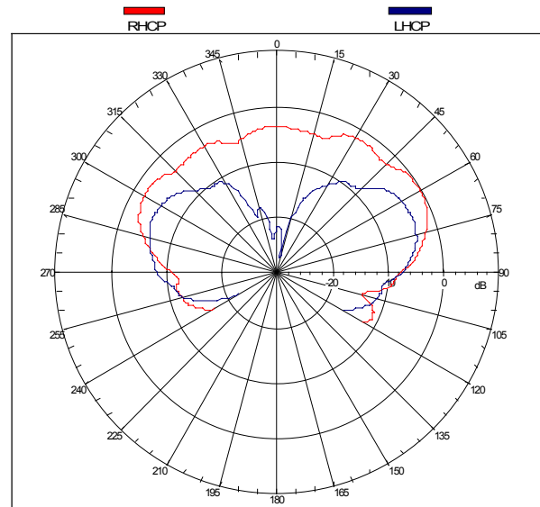
Far-field amplitude of Dsph231a2.nsi
