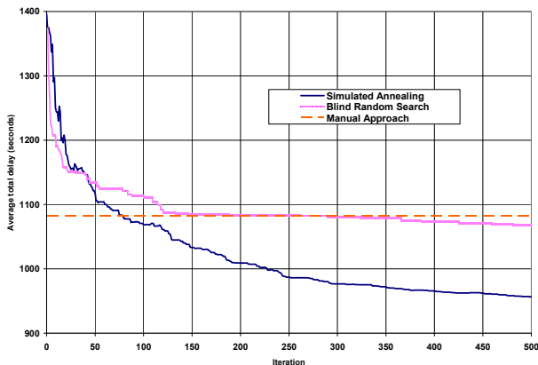
Figure 4: FSAN and Blind Random Search Results
