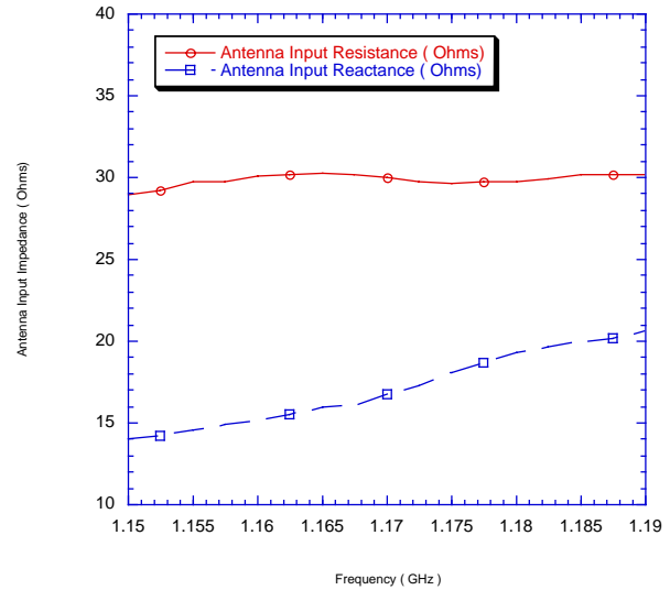
Figure 3a: Measured Input Impedance in the L_5 Band
