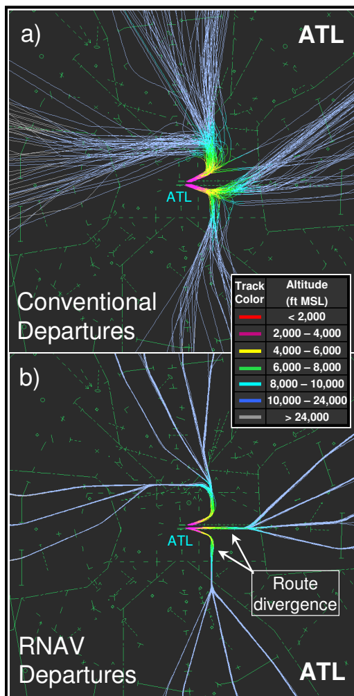
Figure 2. Radar tracks of (a) vectored conventional and (b) non-vectorized RNAV departures in East flow configuration illustrating the route conformance of terminal RNAV operations at ATL.
