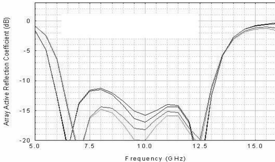
Figure 3. Same Case as Previous Figure but with Some Dielectric Removed Between Elements
