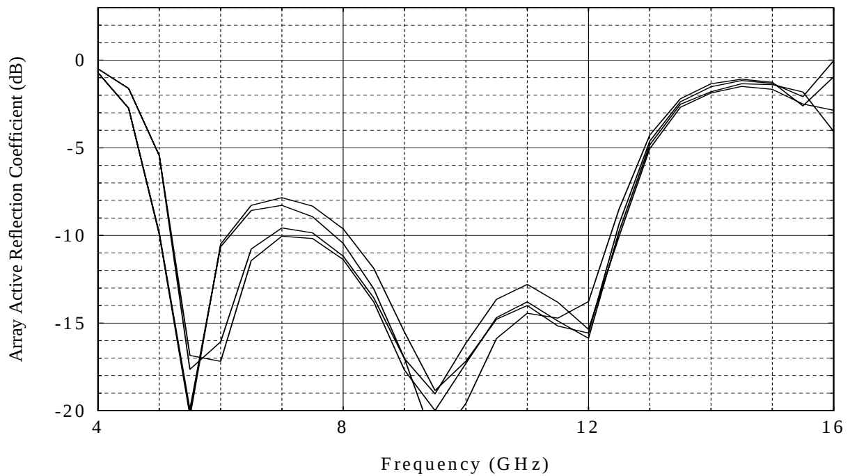
Figure 2. Reflection Coefficient for Broadside Infinite Array, Computed with HFSS. Circular Polarization.
