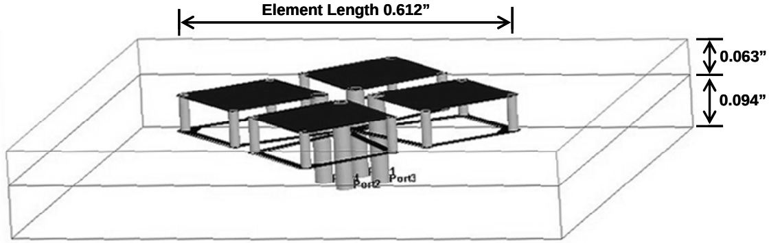
Figure 1. 3D View of One Radiating Element
