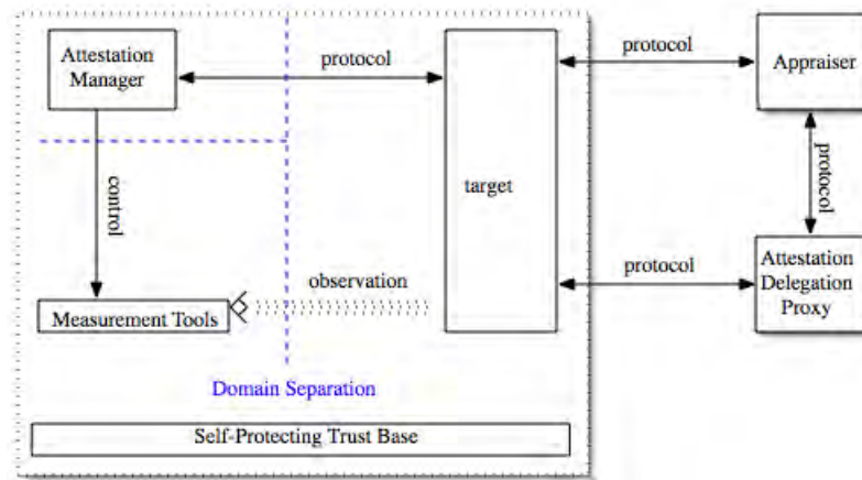
Figure 2: Attestation Architecture
