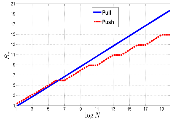
Figure 2. Communication cost comparison between Push and Pull algorithms as a function of N .
