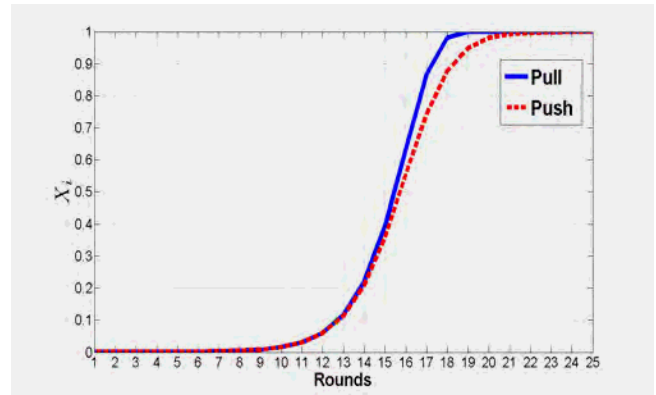
Figure 1. Gossip growth comparison between Push and Pull algorithms for N=2^{15} .
