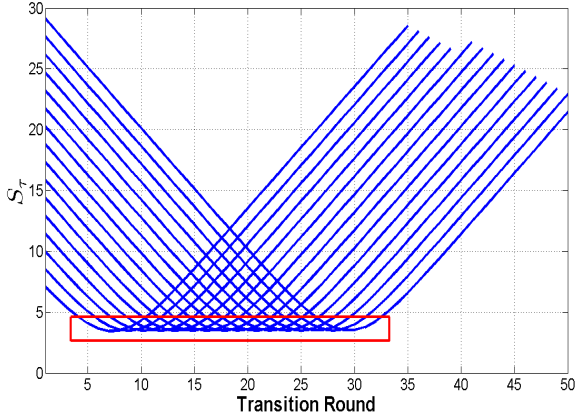
Figure 5. Normalized communication cost for FPTP algorithm as a function of transition round for \alpha = 0.6 .
