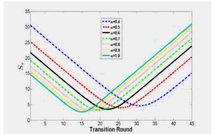
Figure 4. Normalized communication cost for FPTP as a function of transition round for several values of \alpha ( N=2^{15} ).
