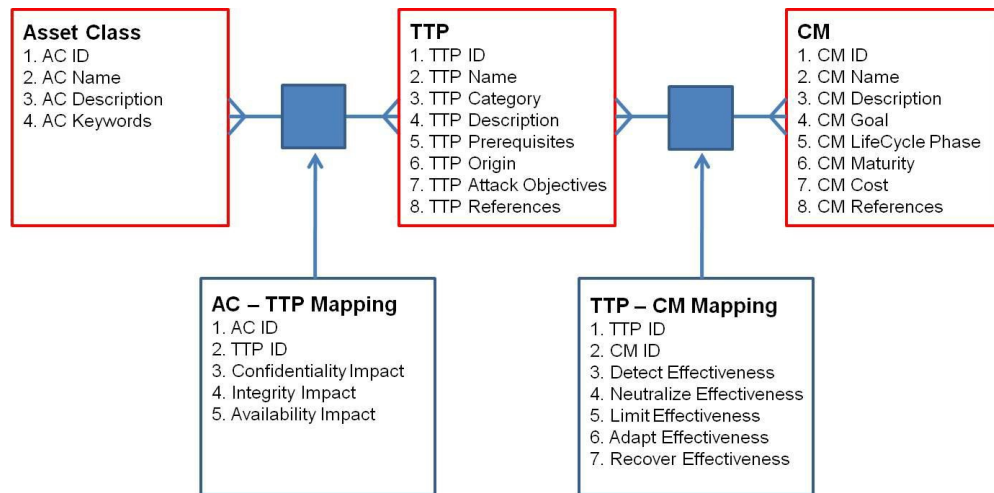
Figure 18 MAE Data Model
