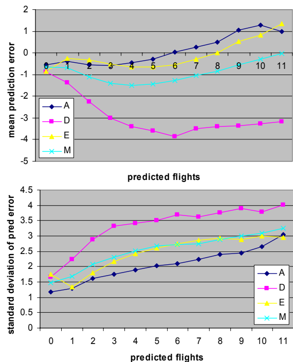
Figure 5: Mean and Standard Deviation of Prediction Errors for 60 min LAT by Sector Type. A = arrival, D = departure, E = en route, M = mixed.
